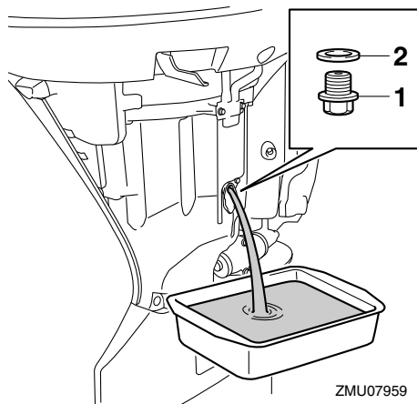
1. Vis de vidange 2. Joint
