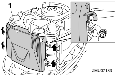
1. ECM (Electronic Control Module) deksel
